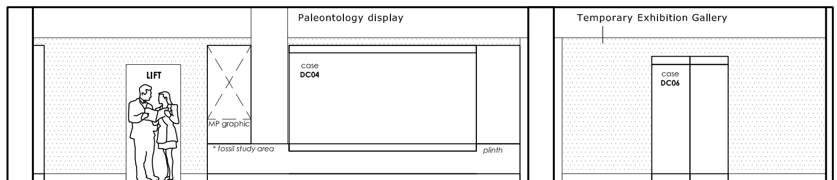
Elevation A-A Paleontology display
