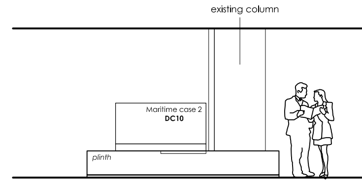
Elevation of Maritime Folkestone plinth
